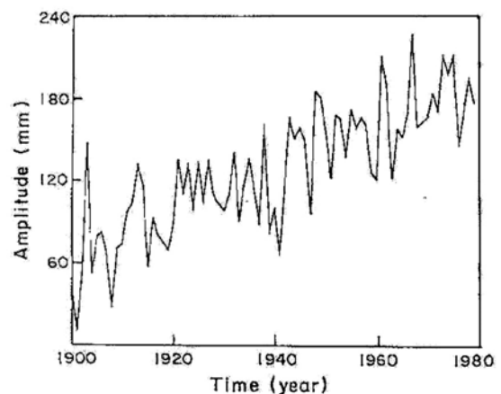
Figure 18: Sea-level (SL) values for 84 tidal-gauge stations with more than 37 years of data [Trupin and Wahr 1990]. They have been corrected for post-glacial rebound. The average rate of rise is ~18 cm per century. Note absence of any acceleration in SL rise during warming intervals. While satellite data [Cazenave and Nerem 2004] suggest a higher rate of rise, an analysis by Holgate [2006] shows a lower rate in recent years.
