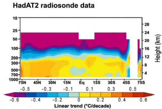
Figure 8: By contrast, observed temperature trends versus latitude and altitude; this is figure 5.7E from CCSP 2006, p. 116. These trends are based on the analysis of radiosonde data by the Hadley Centre and are in good agreement with the corresponding US analyses. Notice the absence of increased temperature trends in the tropical mid-troposphere.
